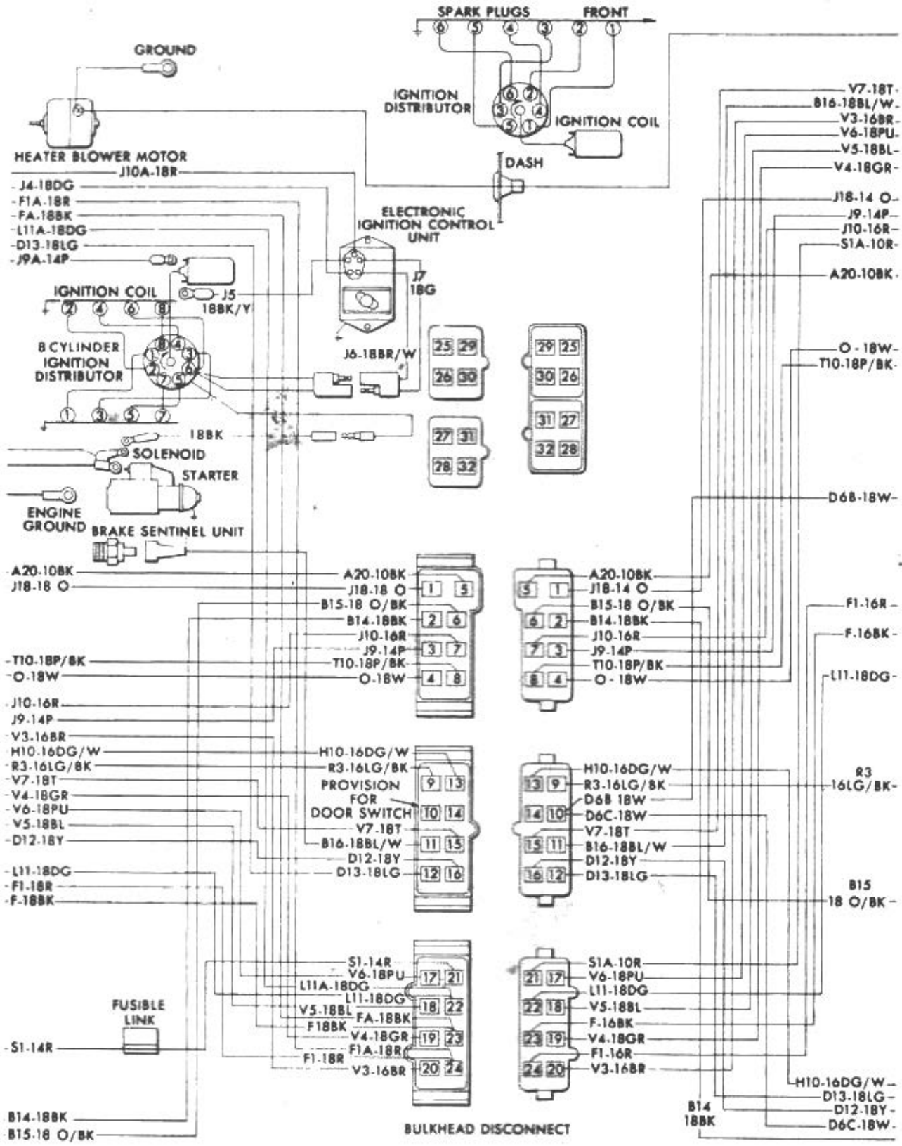
Wiring diagram - 1971 through 1976 models (1977 and 1978 models similar) (2 of 6) Heater, ignition distributor, bulkhead disconnect block
