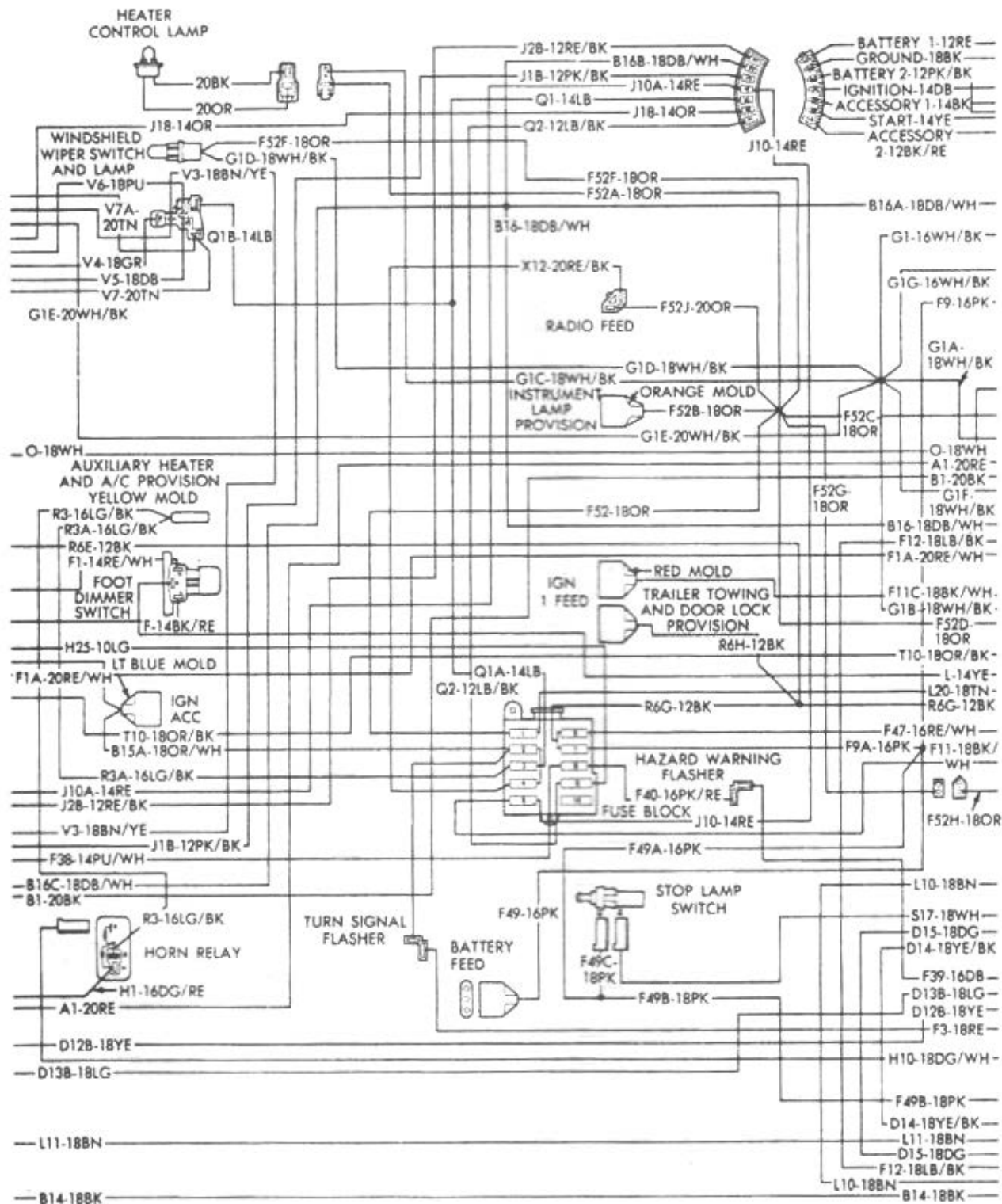
Wiring diagram - 1979 through 1984 models (4 of 6) Fuse block, ignition switch, auxiliary wiring systems
