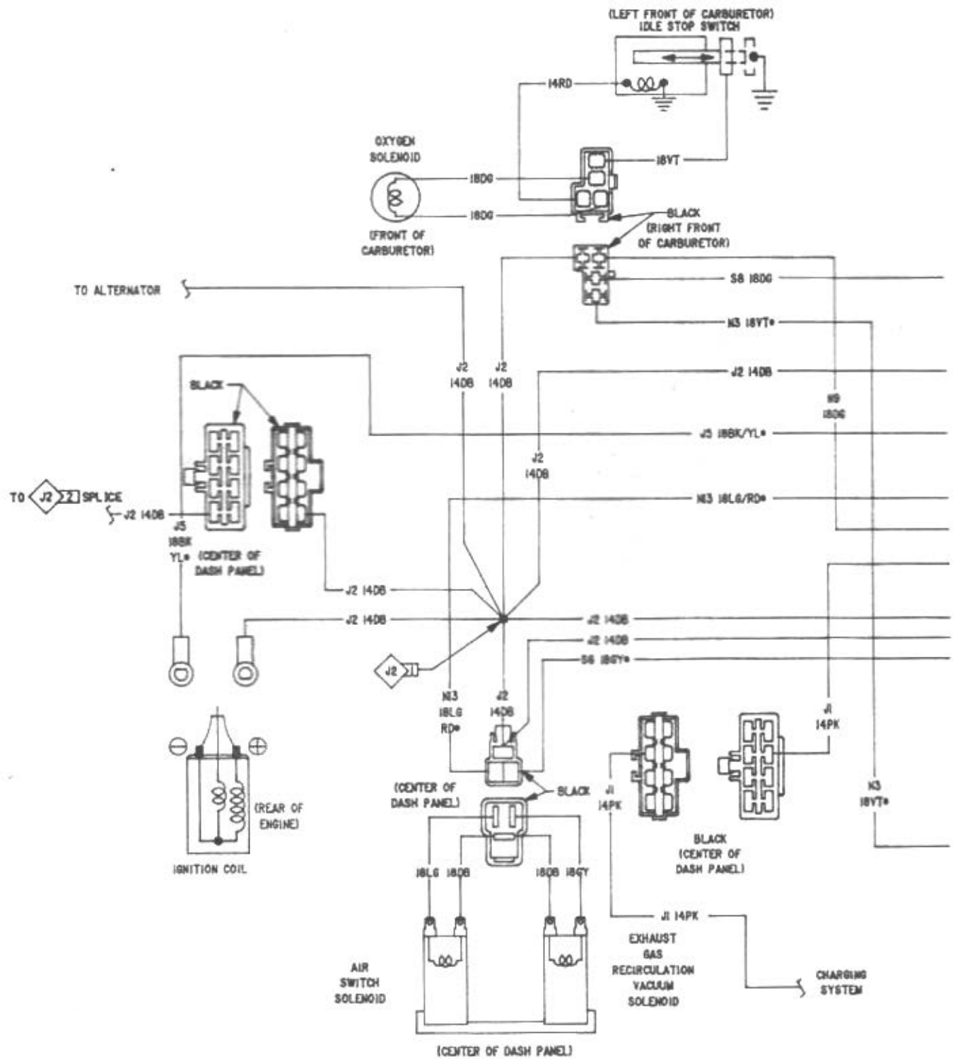
Wiring diagram - 1985 through 1987 models (4 of 11)
