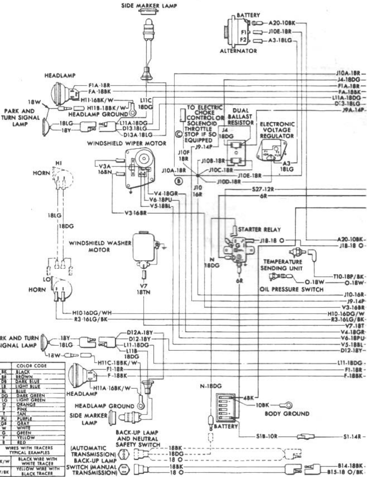
Wiring diagram - 1971 through 1976 models (1977 and 1978 models similar) (1 of 6) Front lights, charging system, starter relay, engine switches
