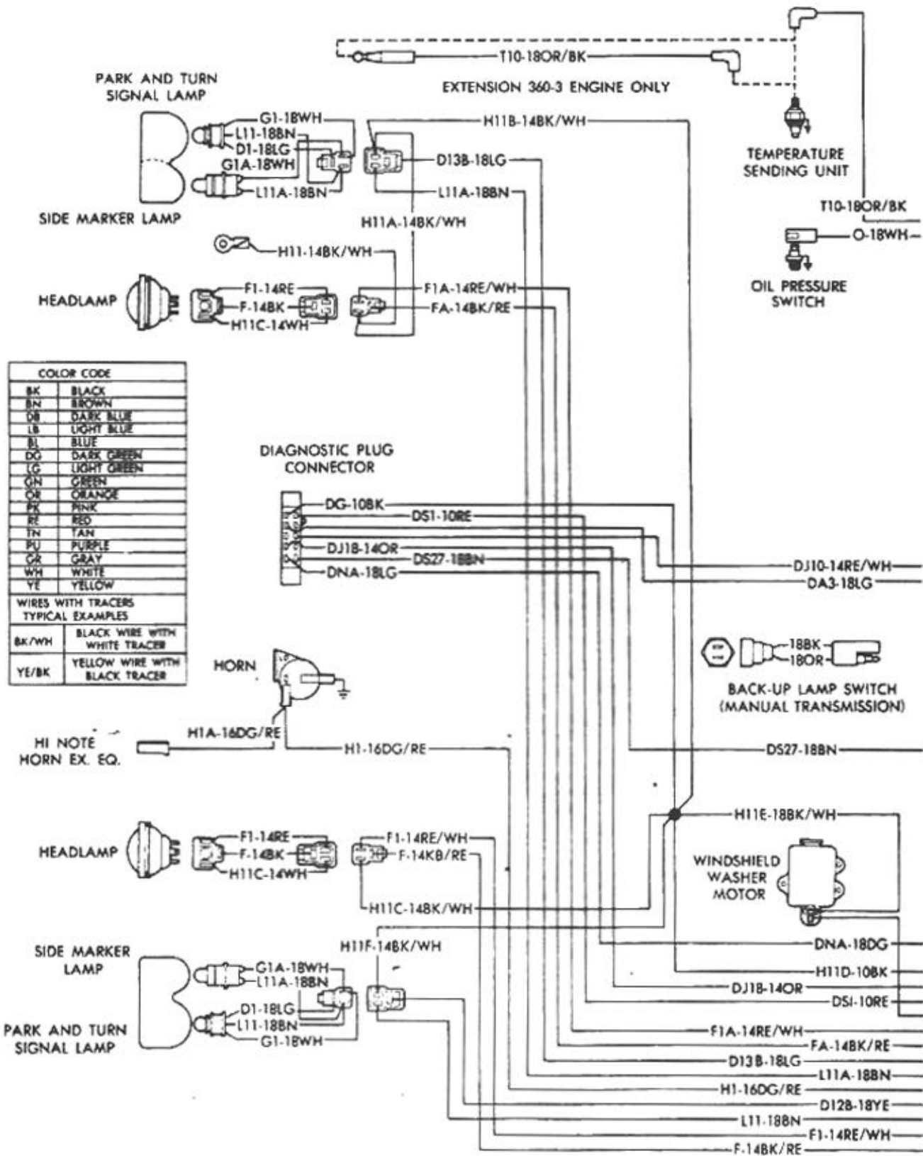
Wiring diagram - 1979 through 1984 models (1 of 6)
