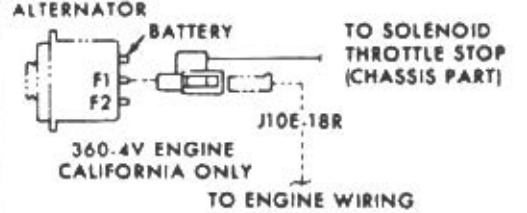
WIRING DIAGRAM ELECTRIC CHOKE CONTROL UNIT AND SOLENOID THROTTLE STOP
