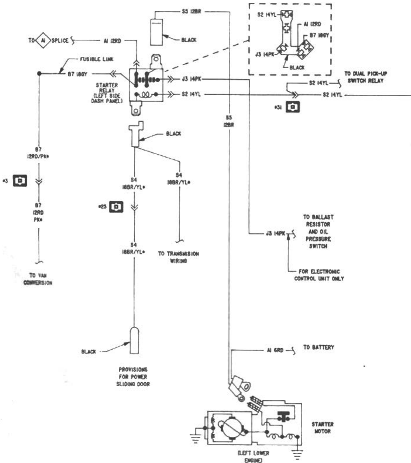
Wiring diagram - 1985 through 1987 models (3 of 11) Starting system
