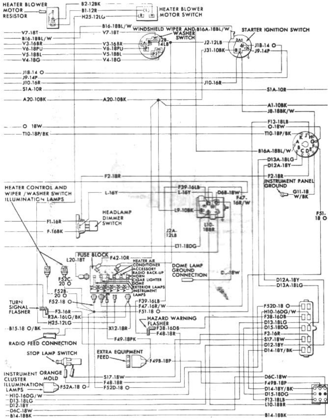
Wiring diagram - 1971 through 1976 models (1977 and 1978 models similar) (3 of 6) Heater, wiper/washer, ignition switch, instrument lights
