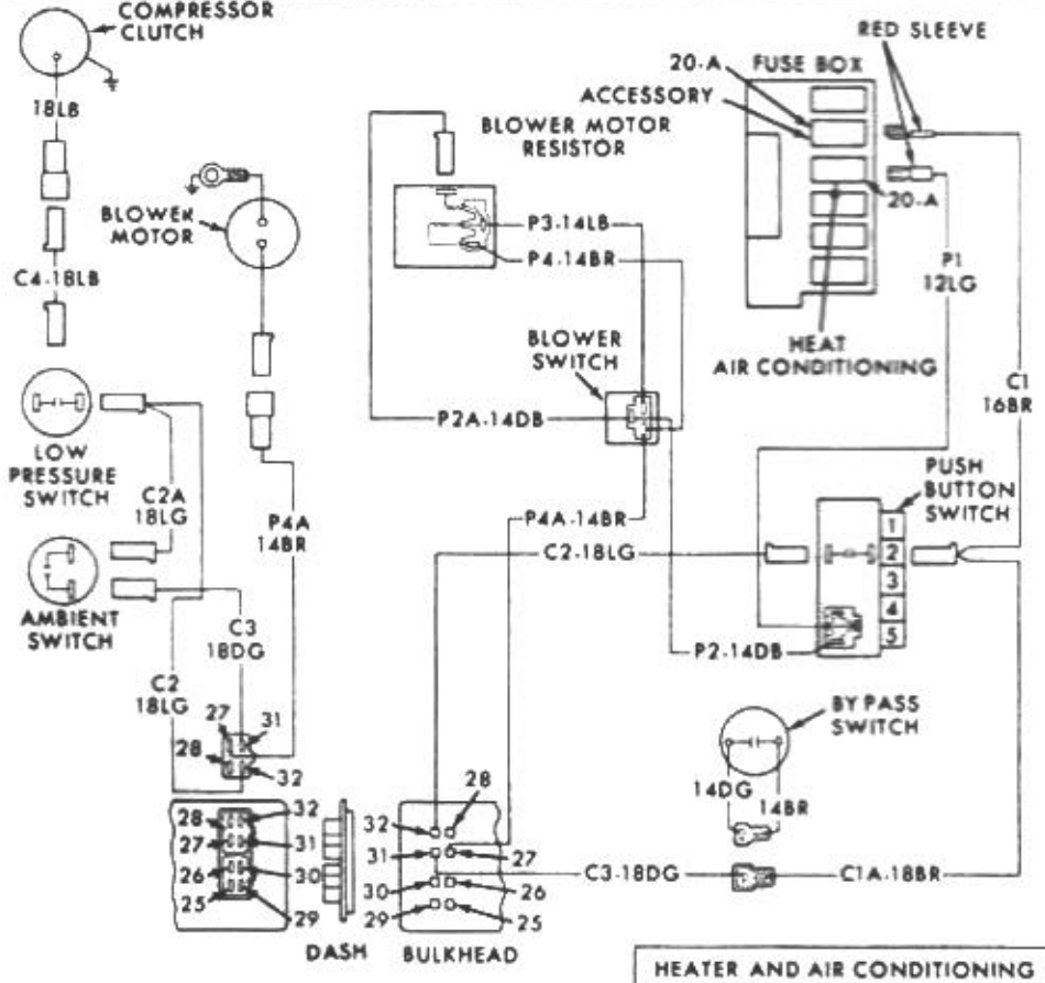
Wiring diagram - 1971 through 1976 models (1977 and 1978 models similar) (6 of 6)
