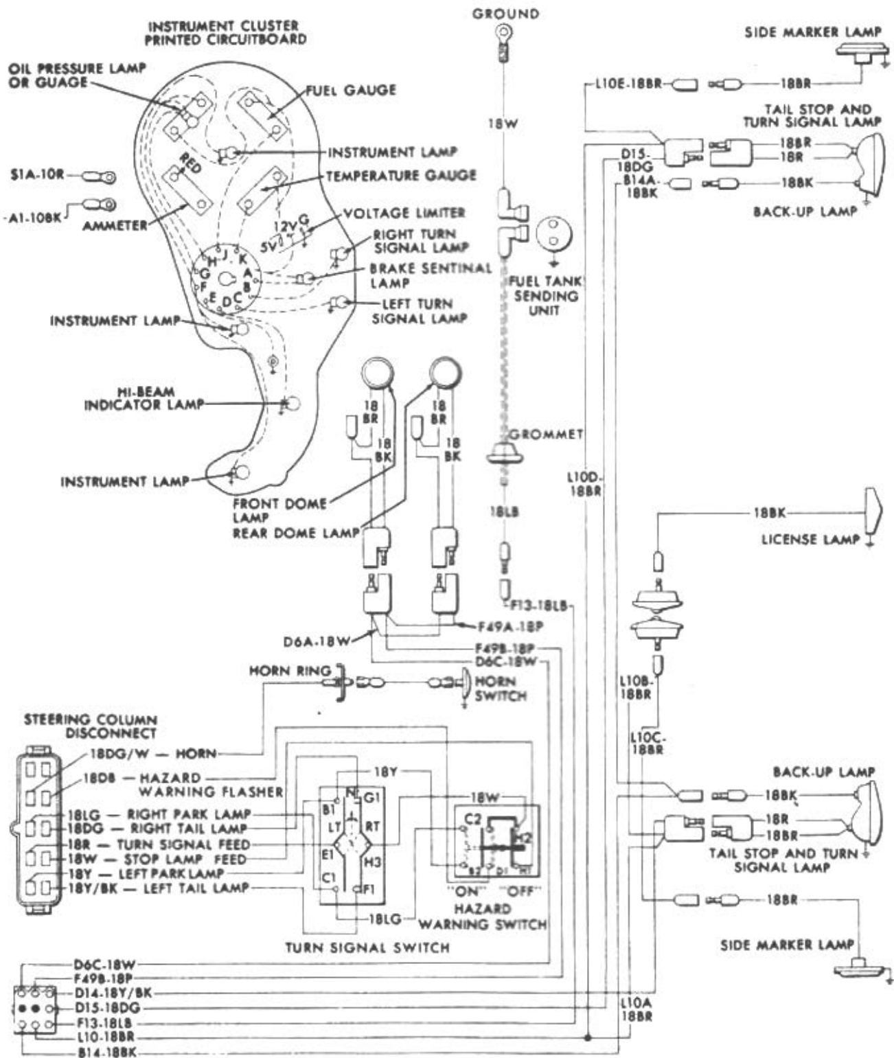
Wiring diagram - 1971 through 1976 models (1977 and 1978 models similar) (4 of 6)
