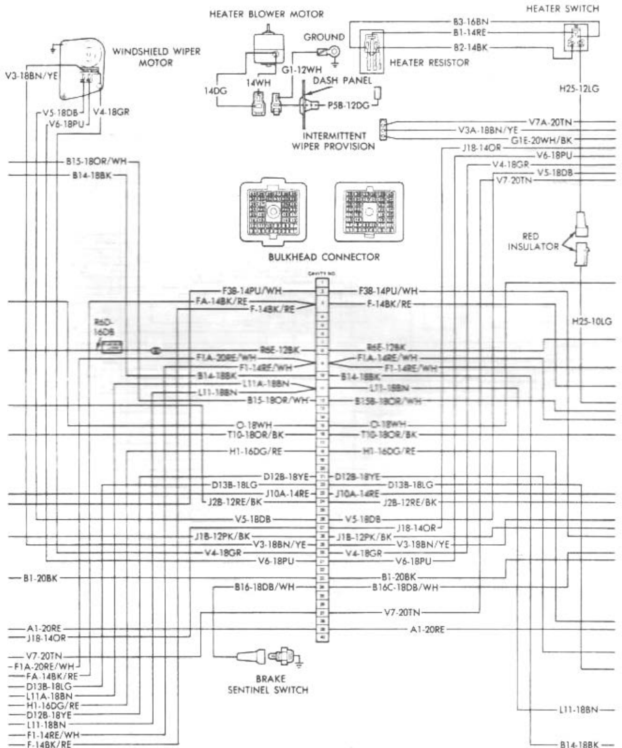
Wiring diagram - 1979 through 1984 models (3 of 6) Heater, wiper motor, bulkhead disconnect block
