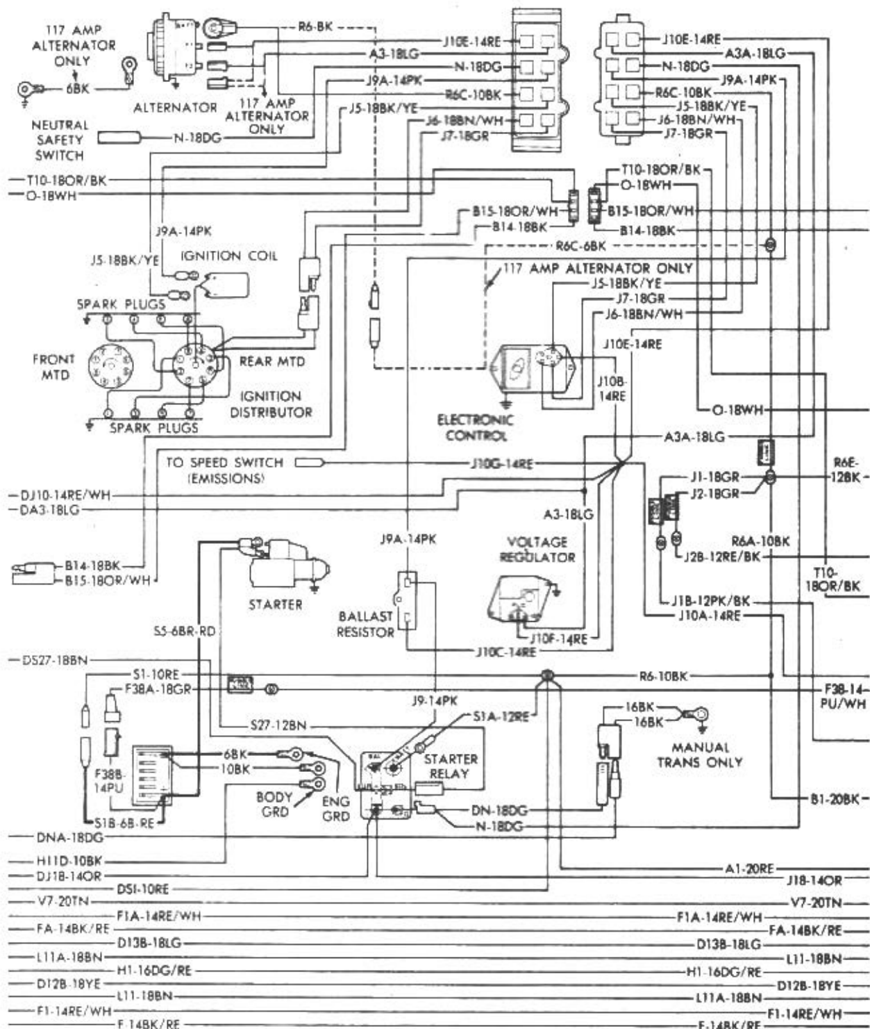
Wiring diagram - 1979 through 1984 models (2 of 6) Charging system, ignition distributor, starting system
