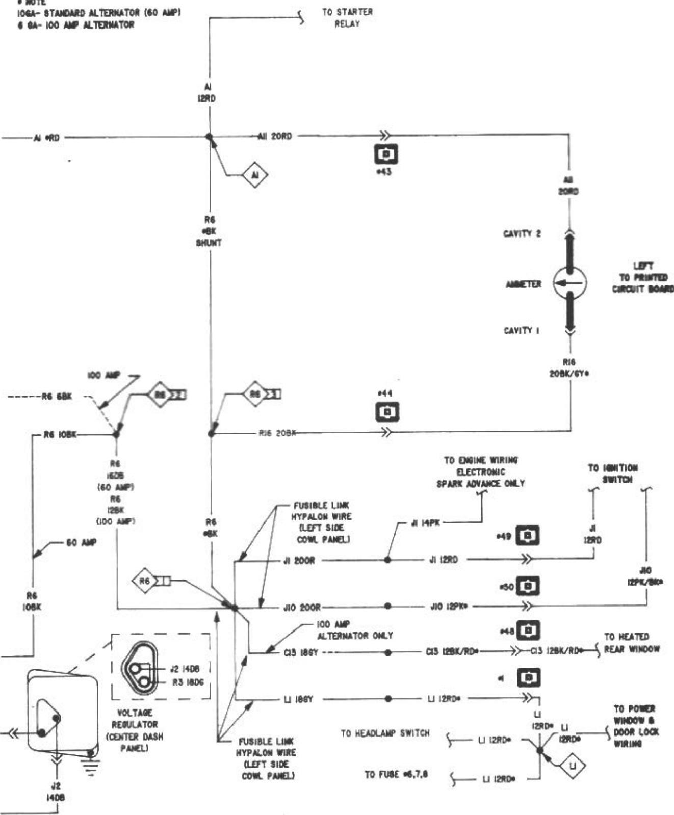
Wiring diagram - 1985 through 1987 models (2 of 11) Charging system
