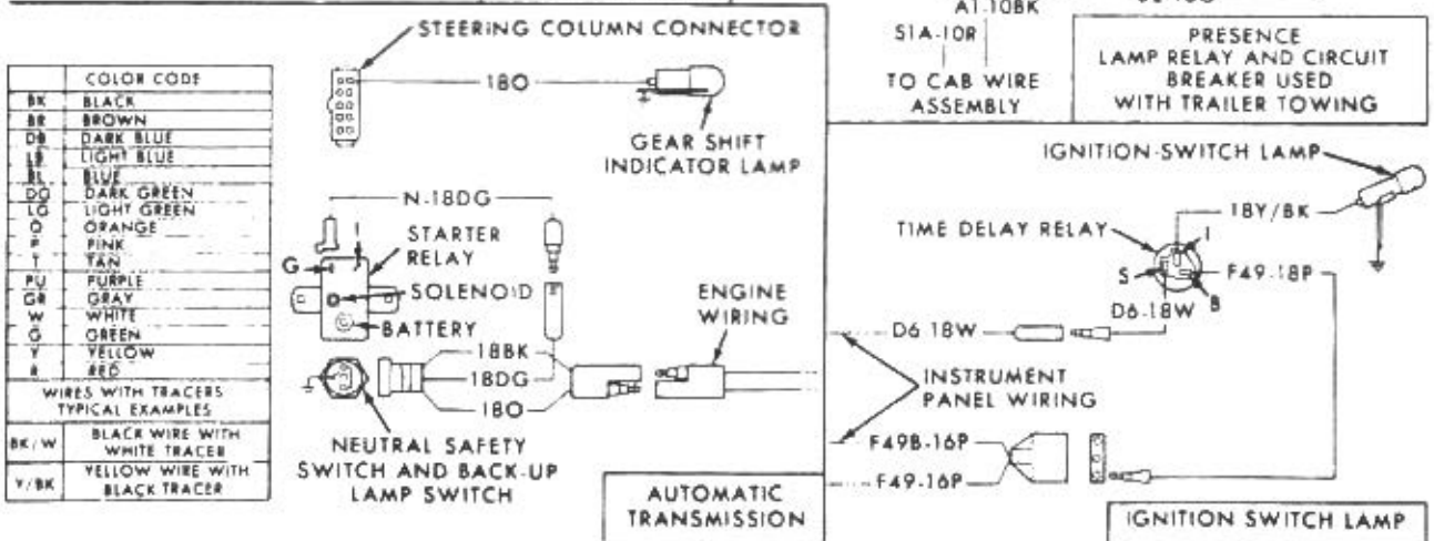
Wiring diagram - 1971 through 1976 models (1977 and 1978 models similar) (5 of 6) Auxiliary wiring systems
