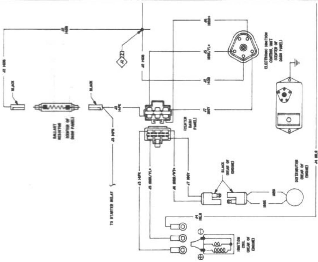
Wiring diagram - 1985 through 1987 models (6 of 11) Electronic control unit - 318/360 V8
