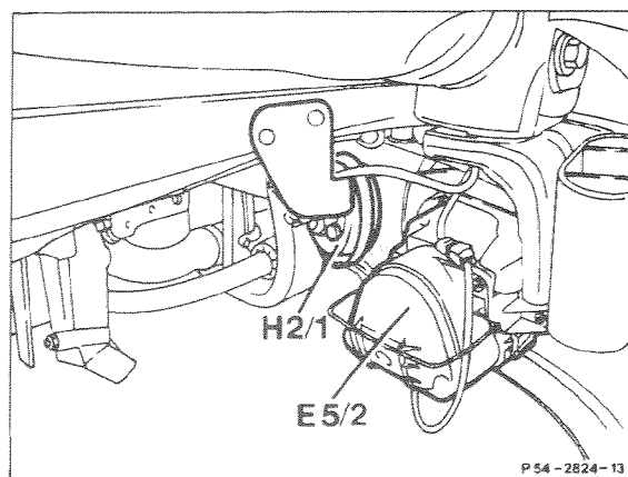
E5/2 Right fog lamp H2/1 Fanfare horn 2
