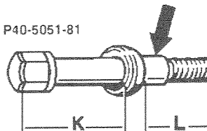
Model 124.036 with fitted shank collar (arrow)
