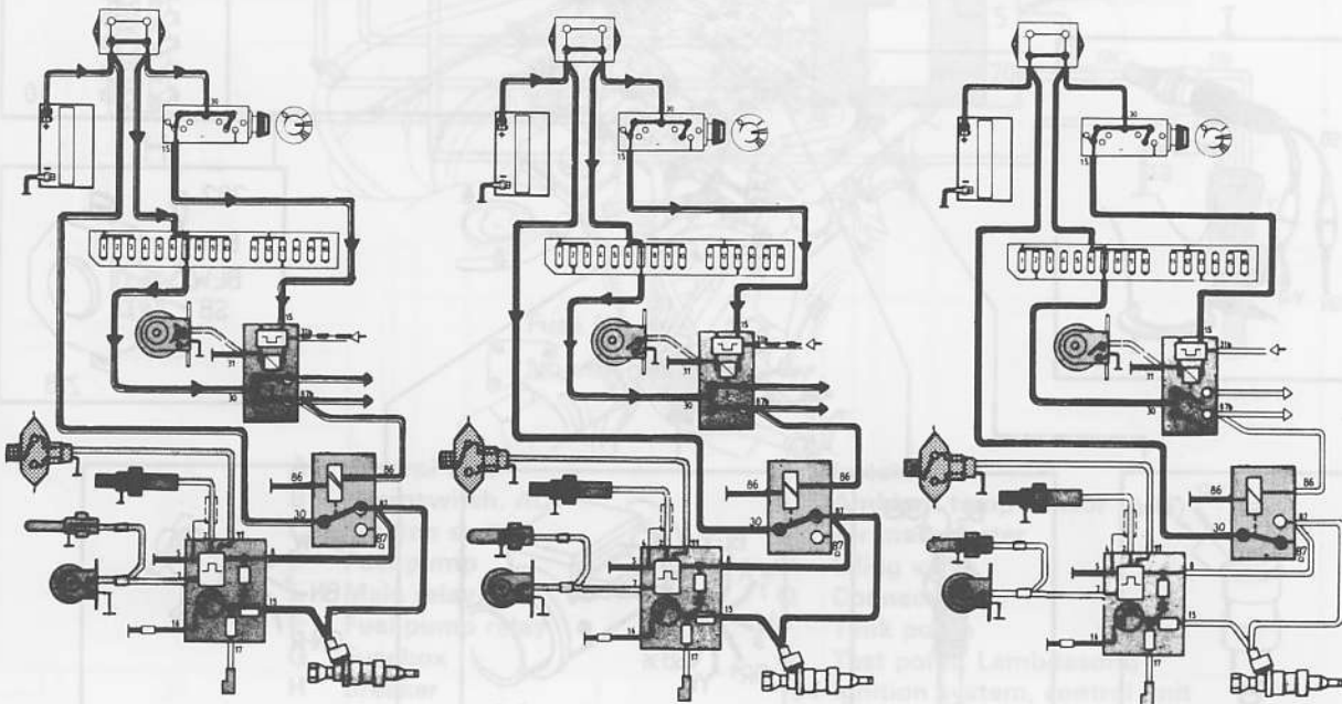
Engine stalled
