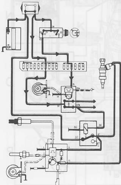
Engine running Frequency valve in duty cycle
